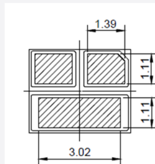
[Recommended PCB Land]
