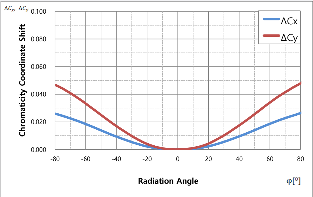
b) Typical Chromaticity Coordinate Shift vs Radiation Angle ( I_F = 1,000\text{ mA} , T_S = 25\text{ }^{\circ}\text{C} ) [7]
