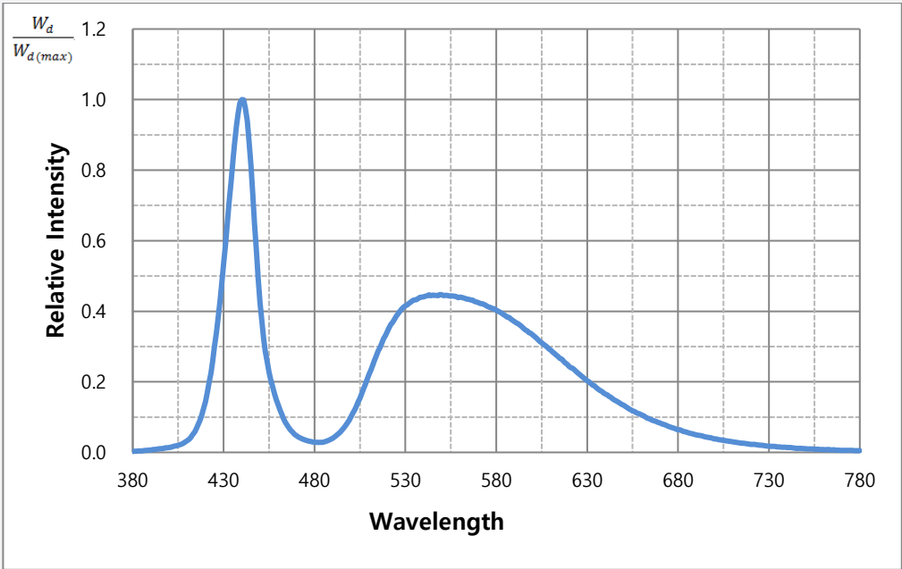
a) Spectrum Distribution ( I_F = 1,000\text{ mA} , T_S = 25\text{ }^{\circ}\text{C} )
