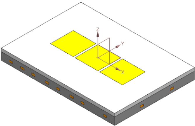
Isometric View
