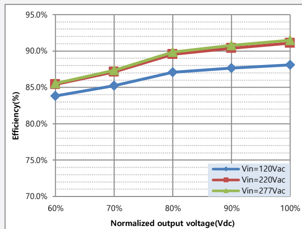
b) Efficiency vs. Load(Iset=5600mA)
