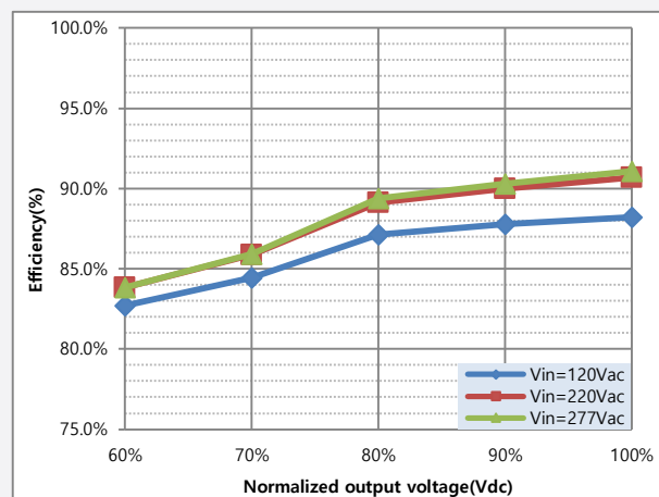
b) Efficiency vs. Load ( I_{set}=6700\text{mA} )
