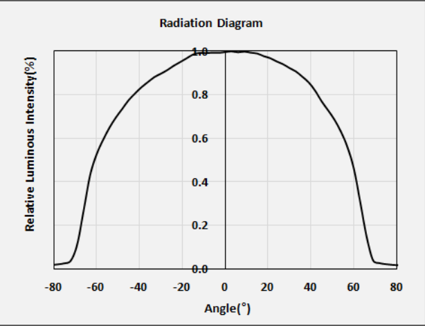
f) Beam Angle Characteristics (If = 350 mA, Tj = 25 °C)
