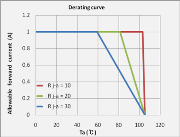
e) Derating Curve and Beam Angle Characteristics (If = 350 mA, Tj = 25 °C)
