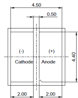
[Bottom View]
