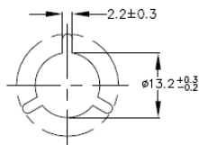
ARBOR HOLE DETAIL A SCALE 2:1
